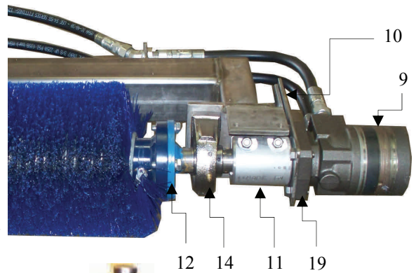
10. TORQUE PLATE
