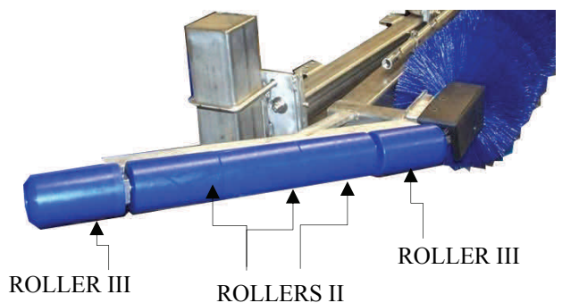
17. ROLLER GUIDE SET—DRIVER SIDE
